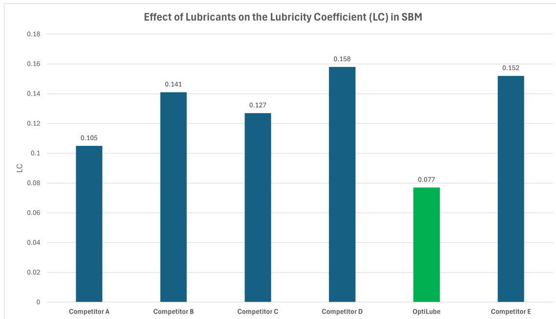
Graph 1 shows independent, third-party lab's findings. OptiLube can be seen in green, while competing lubricants in blue.
